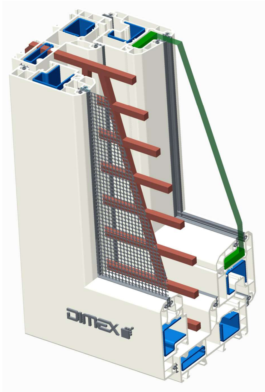
Double Rebate (Double PATAM) Villa Windows Section
