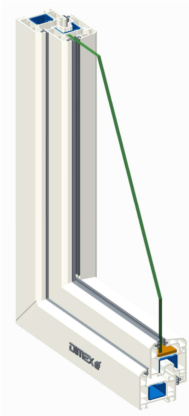
Casement Inward Opening Windows Section
